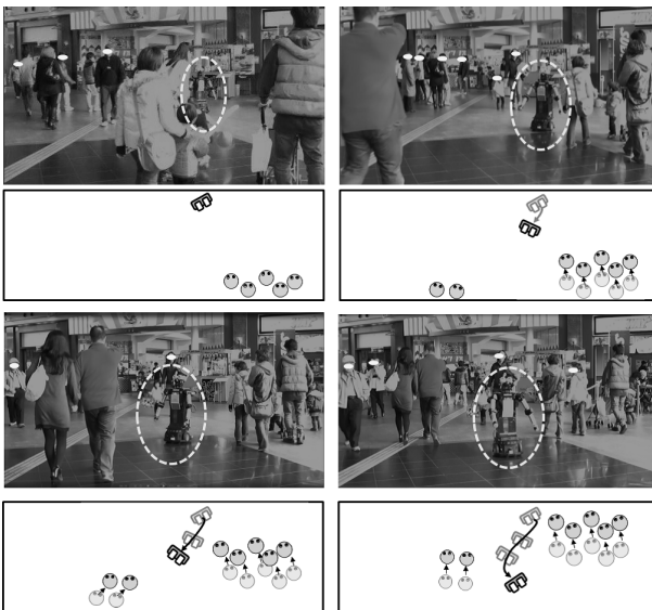
Fig. 9 Video frames and illustration of a situation in which the robot safely navigated through a crowd using the proposed method.
